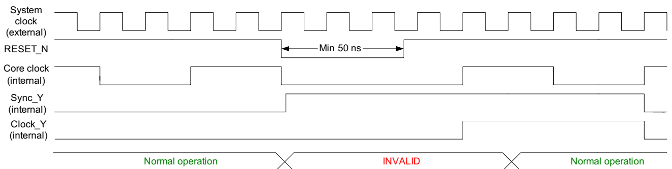
Figure 23. Sequencer Reset Timing
